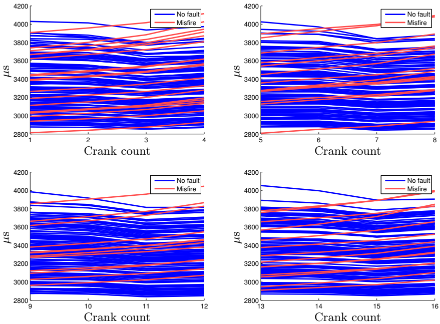
Figure 6: Flywheel angular velocity signal related to cylinder 1, 5, 3 and 6, see Table 3, during normal driving at operating point speed 1500 rpm and load 1.2 g/rev.
