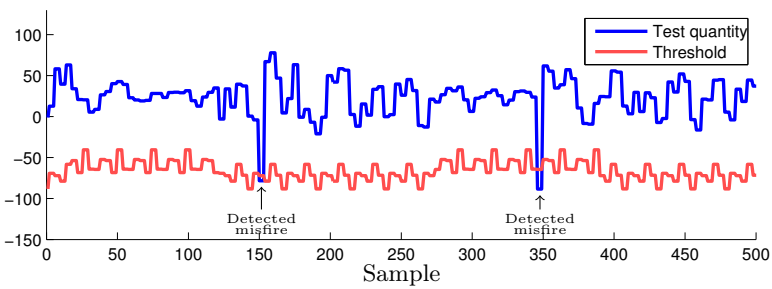
Figure 22: An example of the test quantity and threshold, when maximizing the gap, for a six cylinder engine during normal driving. The threshold variations depends on operating point and cylinder.
