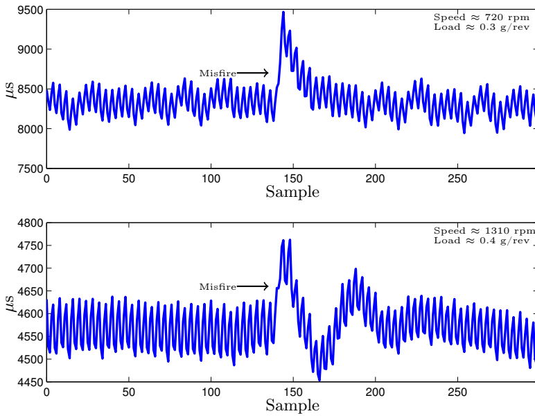
Figure 3: Examples of the flywheel angular velocity signal from a five cylinder engine. The signals contain misfires which are visible as increased measured time.
