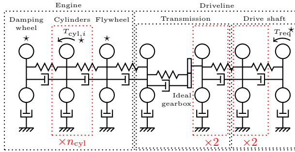
Figure 1: An overview of the model without disturbances. The engine driveline model is composed by a number of connected rotating masses. The connections between the masses are modeled as springs and dampers. The friction at each rotating mass is modeled as a damper connected to ground. The model has n_{\text{cyl}} cylinders where the torque from each cylinder affects a rotating mass of the crankshaft. The gearbox is assumed ideal. Modeled disturbances are marked as stars in the figure.
