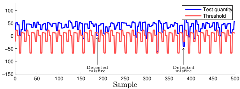
Figure 25: An example of the test quantity and threshold, when maximizing the Kullback-Leibler divergence, for a six cylinder engine during cold start. The threshold variations in the figure depend on the different cylinders.
