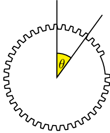
Figure 4: Angular velocity measurements are generated by computing the time difference between two teeth when the flywheel rotates. Two teeth are removed to keep track of the angular position of the flywheel.
