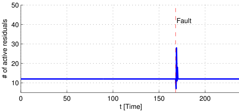
Figure 9: The number of active residuals during a scenario where two sensors fail, f_{24} and f_{35} , occurs at 168 s. The required minimum distinguishability for each residual is lower compared to the result in Figure 8 resulting in fewer active residuals during the scenario. The total number of active residuals during the scenario is 40.
