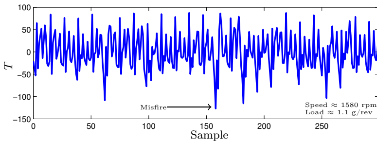
Figure 9: An example of estimated torque during cold start from a six cylinder vehicle. Compared to data in Figure 7, a misfire is more difficult to detect during cold starts.
