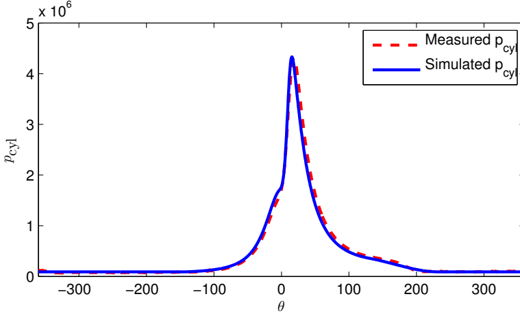
Figure 3: Cylinder pressure model compared to measurement data.
