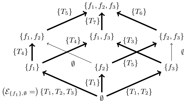
Figure 4: A lattice set representation of all possible candidates for a system with three possible faults. The set at each arrow represents which test quantities that are able to reject d_j for d_i and fulfills a specified distinguishability criteria.
