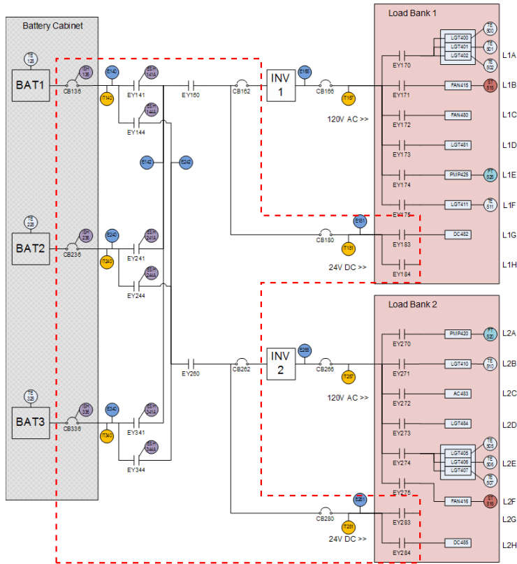
Figure 2: Schematics of the diagnosis test bed ADAPT. The dark area to the left represents the three batteries and the two dark areas to the right are two load banks. Sensors in the circuit are marked as circles. The DC-circuit considered in this work is inside the dotted line.
