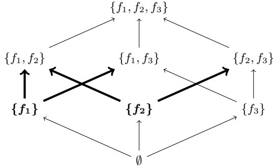
Figure 3: A lattice set representation of all possible candidates for a system with three possible faults where \emptyset corresponds to the fault-free case. If D = \{\{f_1\}, \{f_2\}\} then tests, able to reject \{f_1\} for \{f_1, f_2\} and \{f_1, f_3\} and able to reject \{f_2\} for \{f_1, f_2\} and \{f_2, f_3\} , are needed to improve D .
