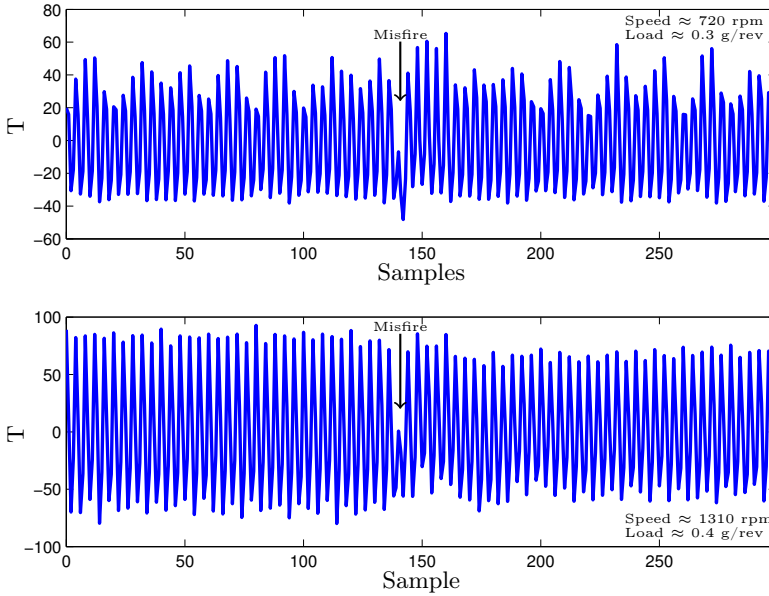
Figure 7: Examples of estimated torque from a five cylinder vehicle. The data contains misfires which are visible as smaller torque gain.
