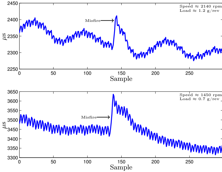
Figure 4: Examples of the flywheel angular velocity signal from a six cylinder engine. The signals contain misfires which are visible as increased measured time.
