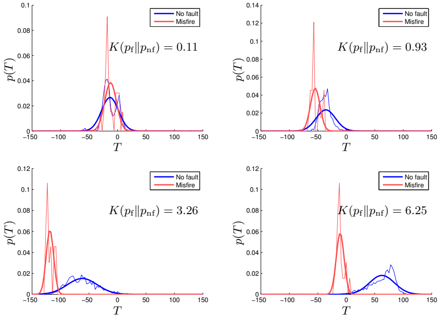
Figure 15: The distribution of the estimated torque of cylinder 1 during cold start at operating point speed 1500 rpm and load 1.2 g/rev. A normalized histogram of the data and an approximation of each distribution as a Gaussian is shown in each plot.
