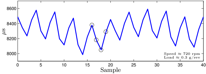
Figure 2: Example of angular velocity measurements at the flywheel from a five cylinder engine. Data related to one combustion from cylinder 3 is marked with circles.
