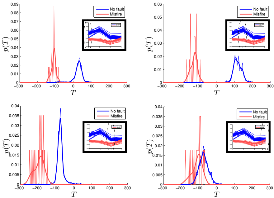
Figure 11: The distribution of the torque of cylinder 1, i.e., crank counts 1, 2, 3, and 4, during normal driving at operating point speed 1500 rpm and load 1.2 g/rev. A normalized histogram of the data and an approximation of each distribution using kernels is shown in each plot. The separation between torque from a fault-free combustion and a misfire is largest at the second sample and smallest at the last sample.
