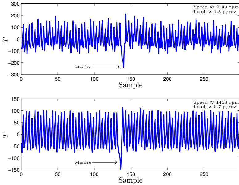
Figure 8: Examples of estimated torque from a six cylinder vehicle. The data contains misfires which are visible as smaller torque gain.
