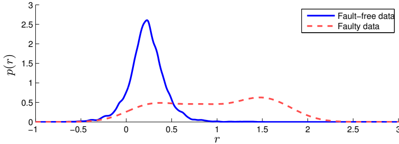
Figure 1.4: Probability density functions of the output y of a residual generator r for the fault-free case and the faulty case.
