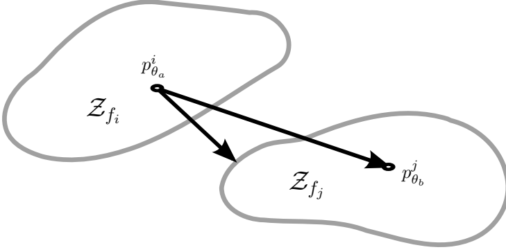
Figure 2: A graphical visualization of the sets \mathcal{Z}_{f_i} and \mathcal{Z}_{f_j} and the smallest difference between p_{\theta_a}^i \in \mathcal{Z}_{f_i} and a pdf p^j \in \mathcal{Z}_{f_j} .
