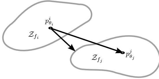
Figure 1: A graphical visualization where the smallest difference between p_{\theta_i}^i \in \mathcal{Z}_{f_i} and a pdf p^j \in \mathcal{Z}_{f_j} is the quantified diagnosability measure.
