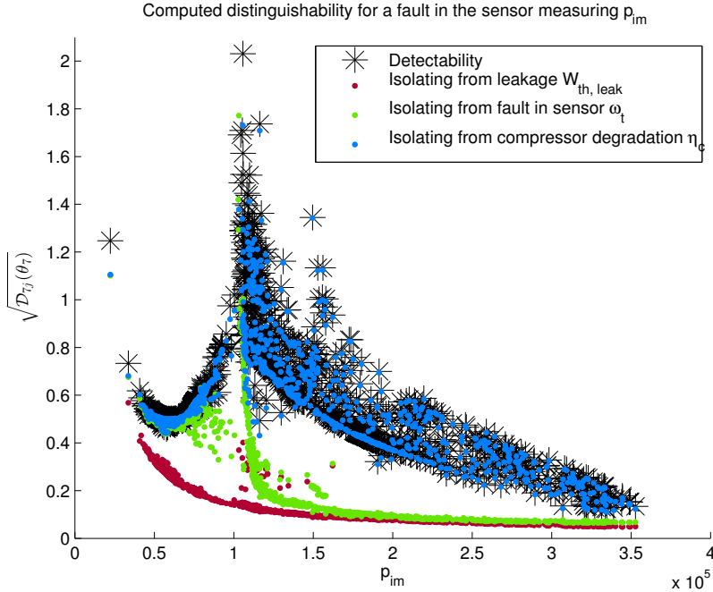
Figure 6: Computed distinguishability for an additive fault in sensor measuring p_{im} . Distinguishability is not changed when isolating from a degradation in the compressor compared to detectability. There is a peak for distinguishability around p_{im} \approx p_{atm} except when isolating from a leakage after the compressor. Distinguishability increases when p_{im} goes to zero because the sensor fault becomes relatively large compared to the measured pressure.
