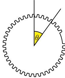
Figure 1: The flywheel angular velocity signal is generated by computing the time difference between two following teeth when the flywheel rotates. Two teeth are removed to keep track of the angular position of the flywheel.
