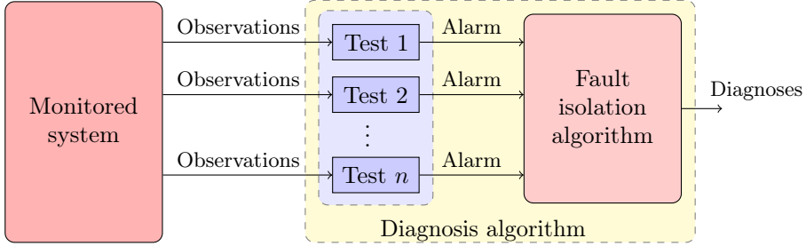
Figure 1.3: An example of a diagnosis algorithm where observations from the system are used to compute possible statements about the system health consistent with the observations, referred to as diagnoses.
