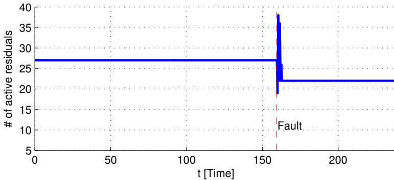
Figure 5: The number of active residuals during a scenario where a relay gets stuck open, f_{10} , occurs at 159 s. The total number of active residuals during the scenario is 64.
