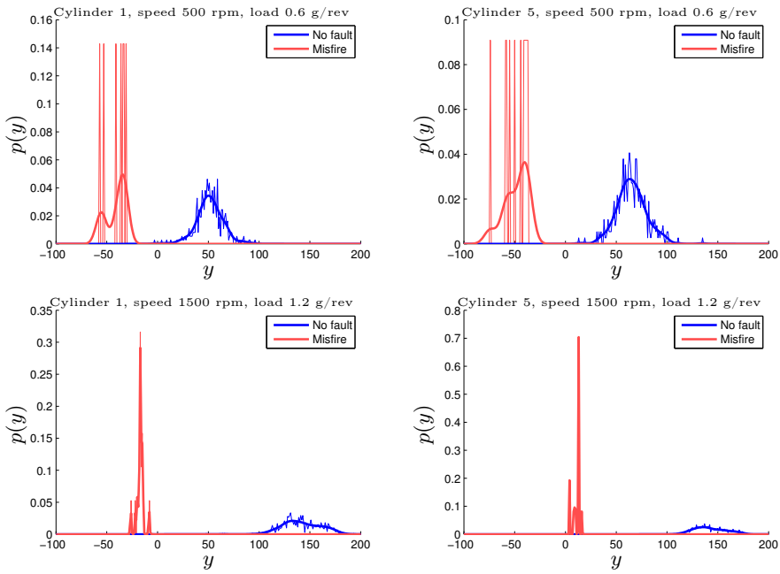
Figure 23: The distribution of the test quantity for different loads and speeds when maximizing the Kullback-Leibler divergence.
