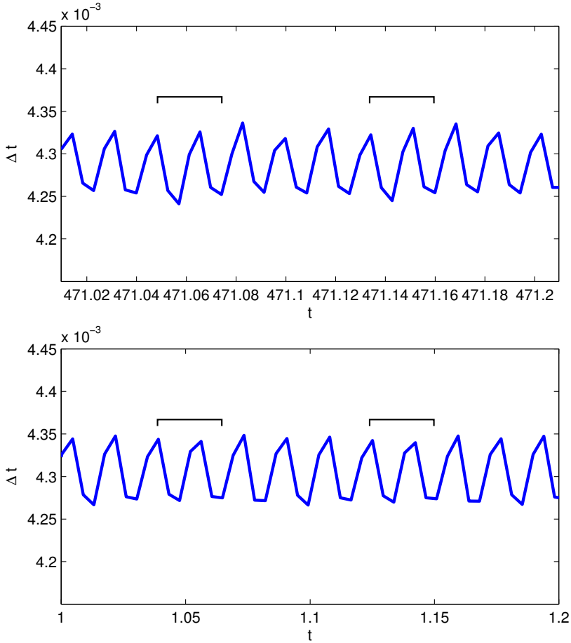
Figure 6: Simulated angular velocity measurements at the flywheel for a five cylinder engine. A qualitative comparison with the real measurement data in Figure 6 shows that the model is able to mimic the behavior of the real data. The cyclic measurement error caused by manufacturing error of the flywheel is marked in the upper figure and a simulation of a similar error in the lower figure.
