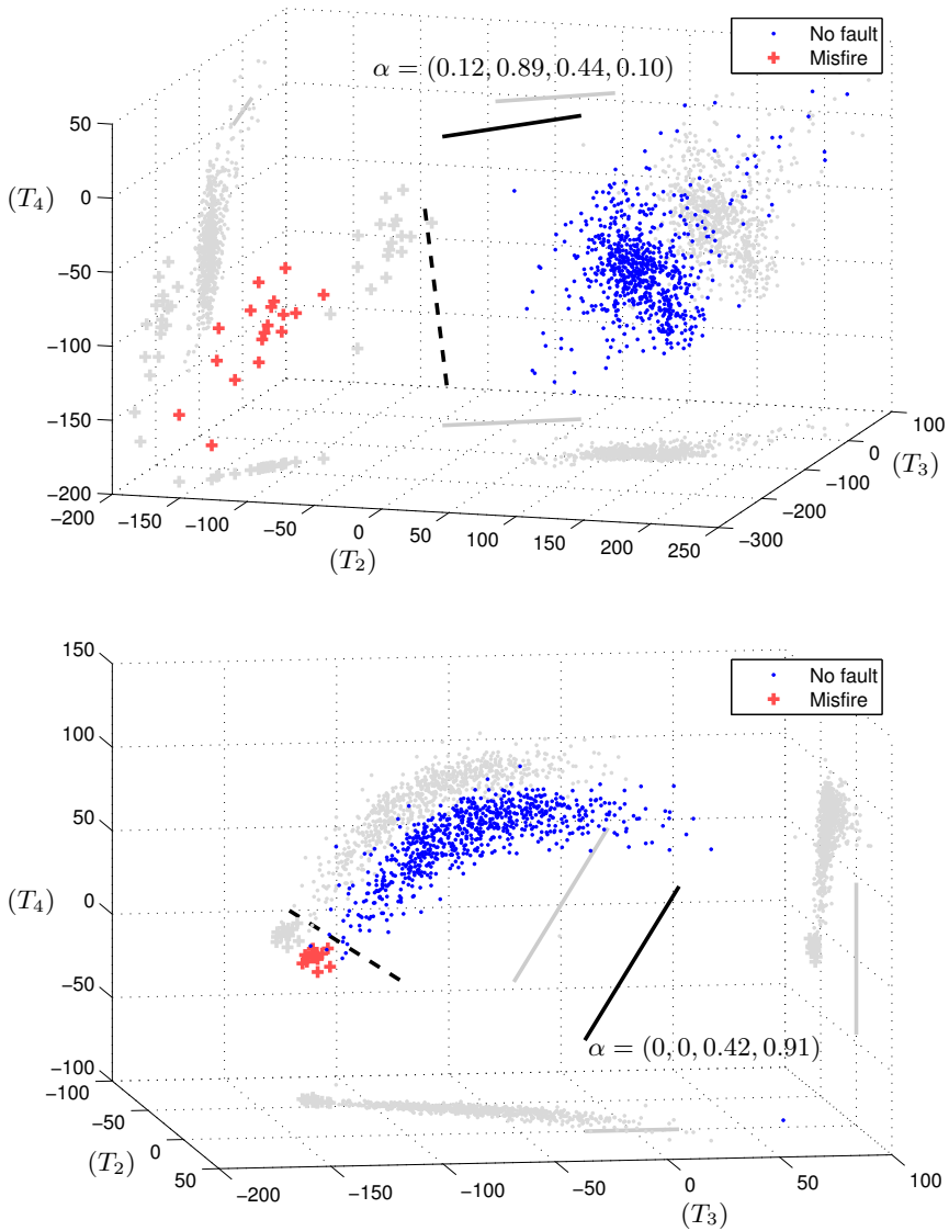
Figure 18: The data in Figure 17 is separated in normal driving, the upper plot, and cold starts, the lower plot. The solid lines represent the weights \alpha such that the distributions of fault-free data and misfire data are well separated. Examples of thresholds to separate fault-free data and misfire data are shown as dashed lines.
