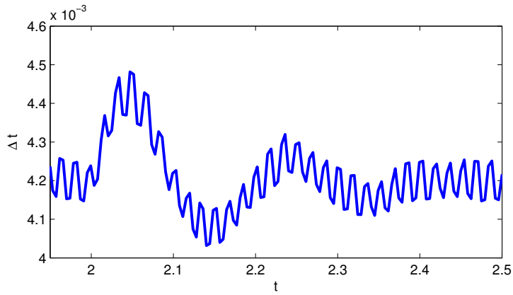
Figure 10: Simulated auxiliary load disturbance at time 2 measured at the flywheel. The auxiliary load is modeled as a step of negative torque at the damping wheel.
