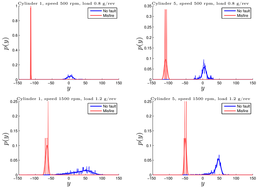
Figure 28: The distribution of the test quantity during cold start for different loads, speeds, and cylinders, when maximizing the gap.
