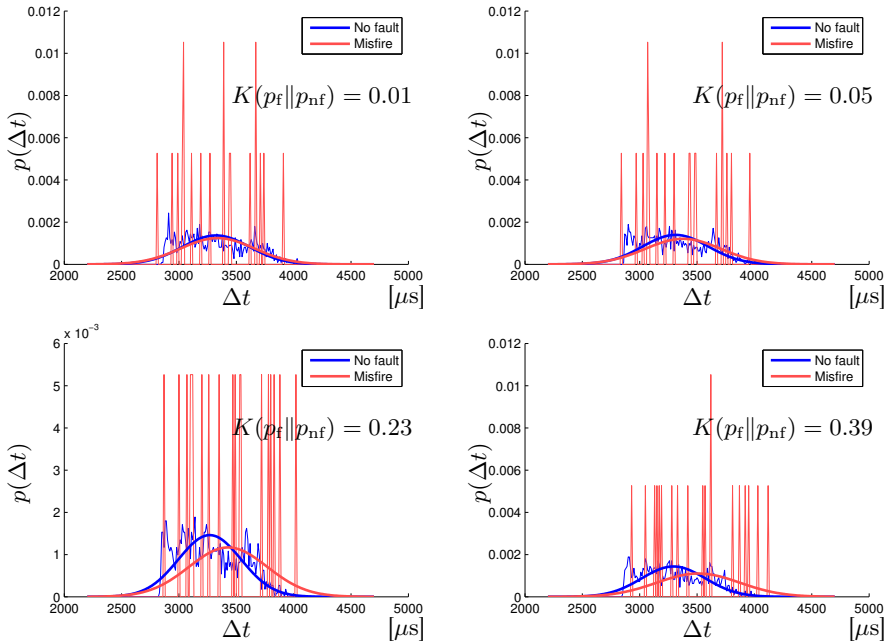
Figure 16: The distribution of the flywheel signal of cylinder 1 during normal driving at operating point speed 1500 rpm and load 1.2 g/rev. A normalized histogram of the data and an approximation of each distribution as a Gaussian is shown in each plot.
