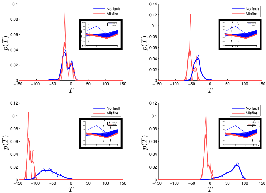
Figure 13: The distribution of the torque of cylinder 1, i.e., crank counts 1, 2, 3, and 4, during cold start at operating point speed 1500 rpm and load 1.2 g/rev. A normalized histogram of the data and an approximation of each distribution using kernels is shown in each plot. The separation between torque from fault-free combustion and a misfire is largest at the last sample and smallest at the first sample.
