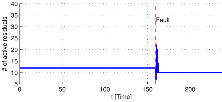
Figure 6: The number of active residuals during a scenario where a relay gets stuck open, f_{10} , occurs at 159 s. The required minimum distinguishability for each residual is lower compared to the result in Figure 5 resulting in fewer active residuals during the scenario. The total number of active residuals during the scenario is 41.
