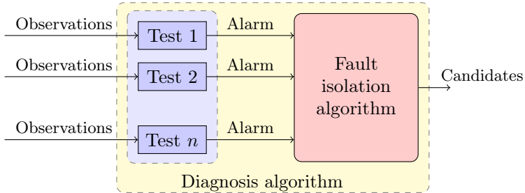
Figure 1: A diagnosis algorithm consists of a set of test quantities and a fault isolation algorithm to compute (minimal) candidates.
