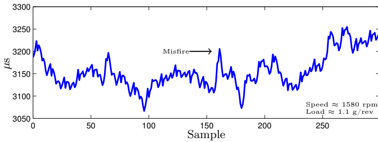
Figure 5: An example of the flywheel angular velocity signal from a six cylinder engine during cold start. Compared to signals in Figure 4, a misfire is more difficult to detect.
