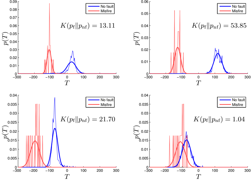
Figure 14: The distribution of the estimated torque of cylinder 1, i.e., crank counts 1, 2, 3, and 4, during normal driving at operating point speed 1500 rpm and load 1.2 g/rev. A normalized histogram of the data and an approximation of each distribution as a Gaussian is shown in each plot.
