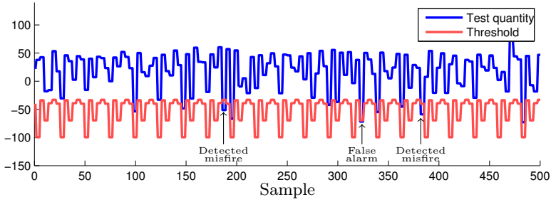
Figure 26: An example of the test quantity and threshold, when maximizing the gap, for a six cylinder engine during cold start. The threshold variations in the figure depend on the different cylinders.
