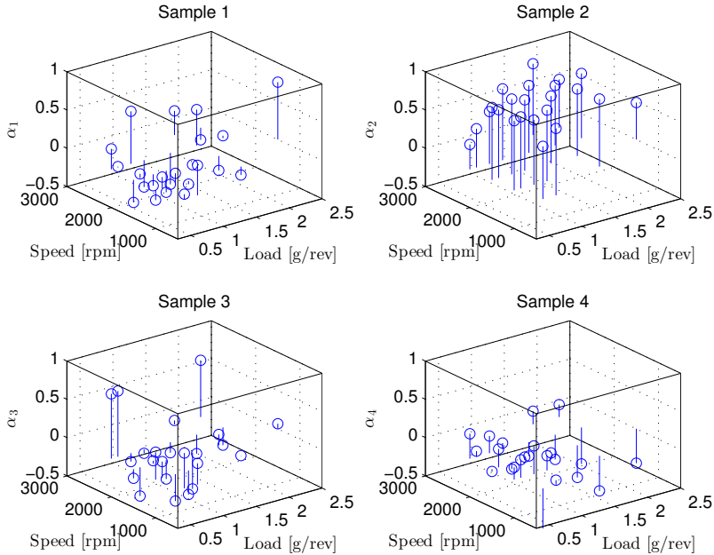
Figure 19: Optimized weights \alpha for samples from cylinder 1 which maximizes the Kullback-Leibler divergence from the misfire distribution to the fault-free distribution.
