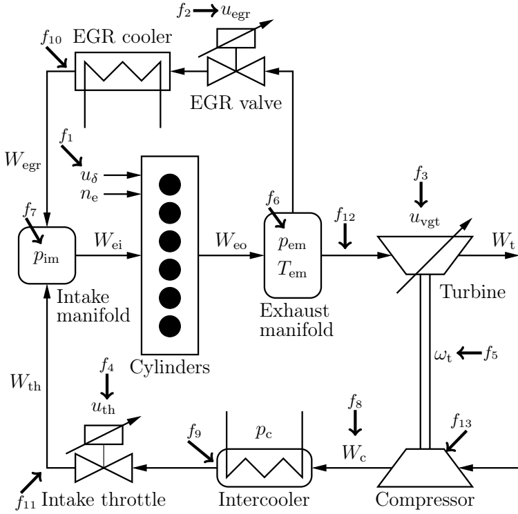
Figure 4: Overview of diesel engine model. The arrows indicate the locations in the model of the modeled faults in Table 6.
