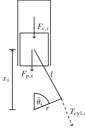
Figure 2: The cylinder model describes cylinder torque T_{\text{cyl},i} as a function of compression pressure force F_{c,i} and the piston mass force F_{p,i} .
