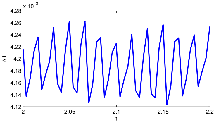
Figure 7: Errors have been added to the teeth angles where measurements on the flywheel are made.
