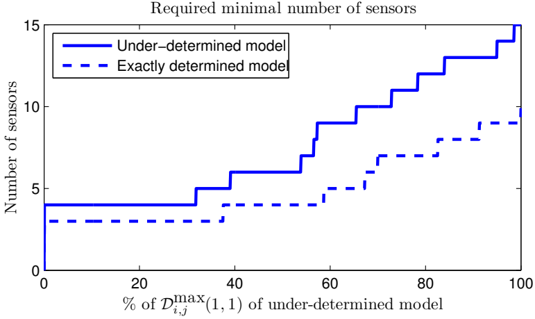
Figure 4: The least number of sensors required to exceed a certain percentage of maximum distinguishability given the underdetermined model described in Figure 3, for the underdetermined case and the exactly determined case, given a global search.
