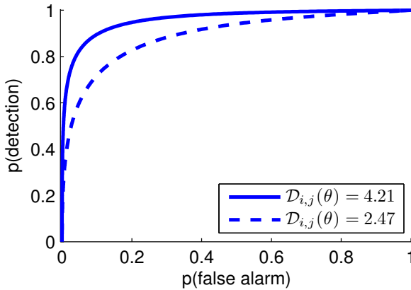
Figure 3: A ROC-curve comparing probability of detection and false alarm for two residuals with different computed values of distinguishability. A higher distinguishability corresponds to a higher ratio between the probability of detection and false alarm.
