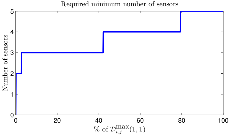
Figure 2: The least number of sensors required to exceed a certain percentage of maximum distinguishability given the example model (1). Note that the number of sensors when required performance goes to zero is equal to the cardinality of the minimal sensor sets (2) from the structural analysis.
