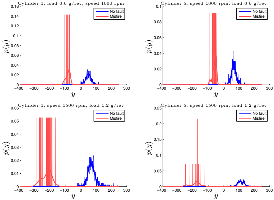
Figure 24: The distribution of the test quantity for different loads, speeds, and cylinders, when maximizing the gap.
