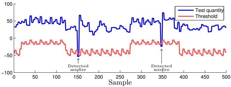
Figure 21: An example of the test quantity and threshold, when maximizing the Kullback-Leibler divergence, for a six cylinder engine during normal driving. The threshold variations depends on operating point and cylinder.
