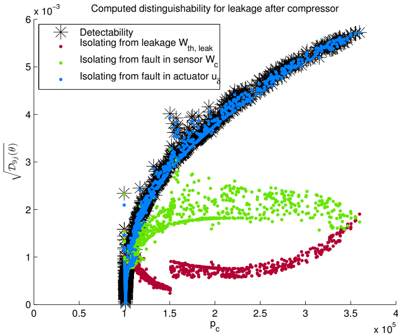
Figure 5: Computed distinguishability for a leakage after the compressor. Distinguishability for a leakage after the compressor from the no fault case, i.e., detectability performance, increases by increasing compressor pressure. Isolating the leakage from a leakage after the throttle, or a fault in the sensor measuring the mass flow through the compressor, affects the performance negatively while isolating from a fault in control signal u_\delta does not affect the performance noticeably.
