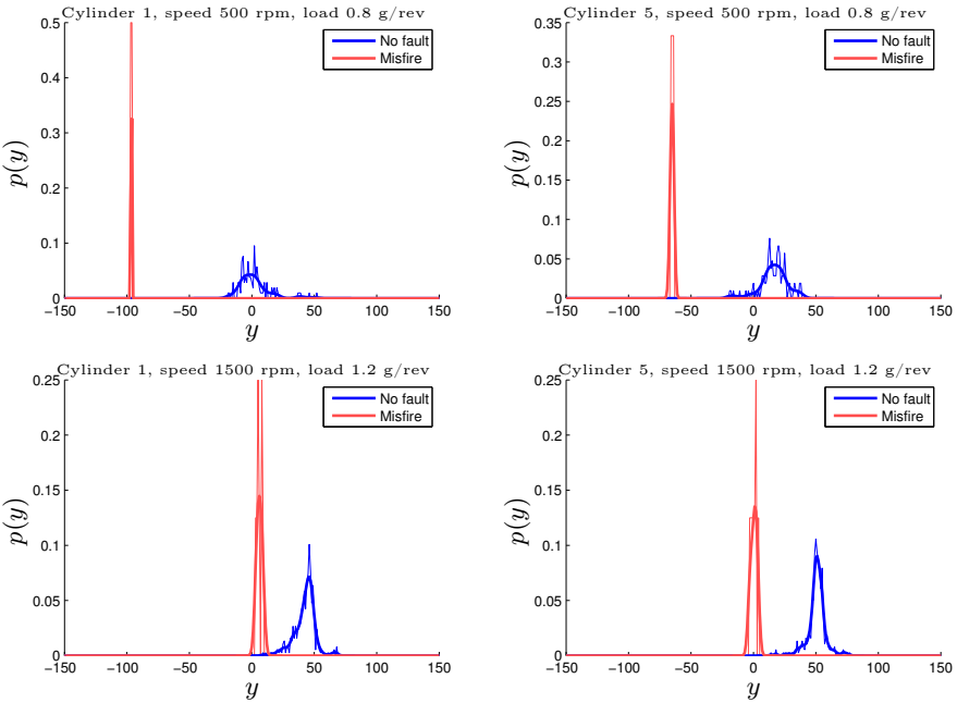
Figure 27: The distribution of the test quantity during cold start for different loads and speeds when maximizing the Kullback-Leibler divergence.
