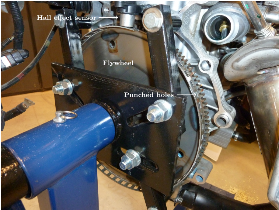
Figure 1.5: A picture of a flywheel and the Hall effect sensor.
