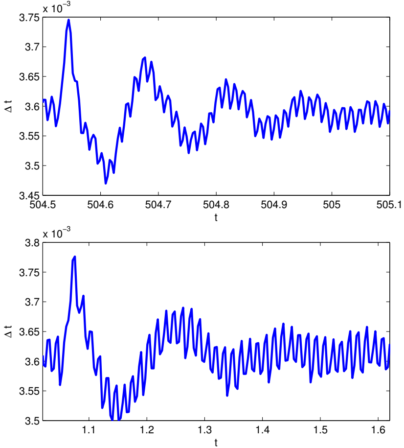
Figure 8: In the lower figure simulated angular velocity measurements at the flywheel are shown during a misfire and in the upper figure real measured angular velocity during a misfire.
