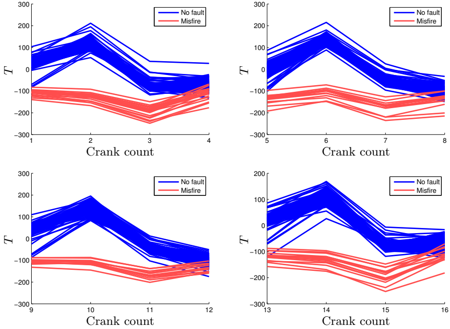
Figure 10: Estimated torque of cylinder 1, 5, 3, and 6 during normal driving at operating point speed 1500 rpm and load 1.2 g/rev.
