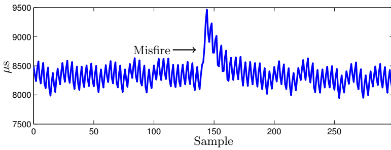
Figure 1.6: Flywheel angular velocity signal when a misfire occurs.
