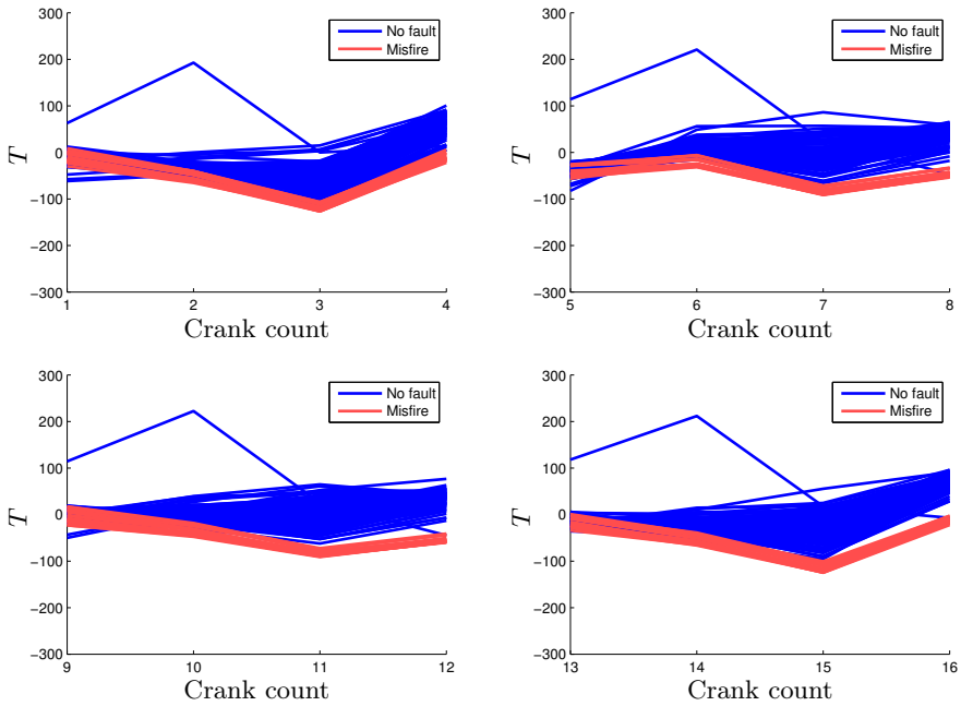
Figure 12: Estimated torque of cylinder 1, 5, 3, and 6 during cold start at operating point speed 1500 rpm and load 1.2 g/rev.
