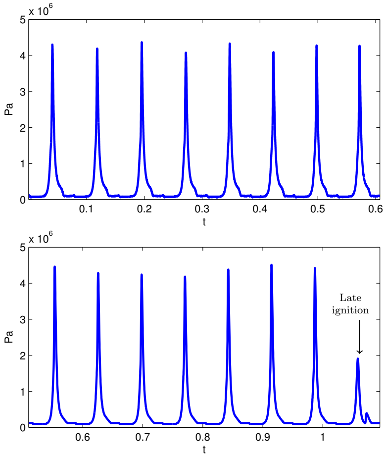
Figure 5: Measured cylinder pressure in one cylinder in the upper figure compared to simulated cylinder pressure with varying ignition angle in the lower figure. The last peak is a simulated late ignition
