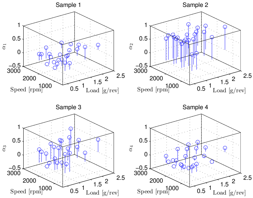
Figure 20: Optimized weights \alpha for samples from cylinder 1 which maximizes the gap between the fault-free and misfire distributions.
